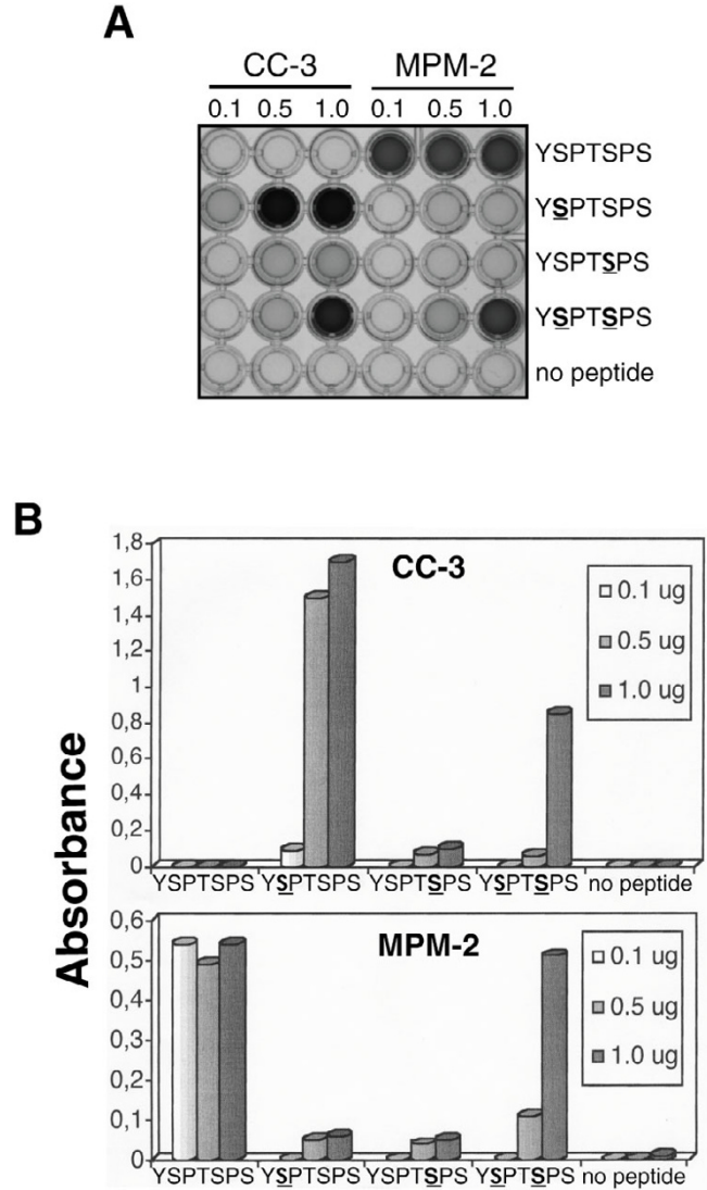
Figure 3 Fine mapping of CC-3 and MPM-2 epitopes on Rpb1 consensus heptad repeats. (A) Biotinylated CTD peptides were immobilized on a streptavidin-coated ELISA plate at three different concentrations and incubated with MPM-2 and CC-3. These peptides contained four YSPTSPS repeats, phosphorylated either on the serine residues at position 2 (Y S PTSPS), at position 5 (YSPT S PS) or at both positions (Y S PT S PS). An unphosphorylated peptide was used as a control (YSPTSPS). CC-3 was mainly reactive with peptides phosphorylated on serine 2 of the consensus repeat whereas MPM-2 reacts preferentially with the peptide phosphorylated on both serines 2 and 5. Surprisingly, MPM-2 also reacted with the unphosphorylated peptide in a concentration independent manner (see text). (B) Histogram of the CC-3 and MPM-2 reactivities shown in (A).
