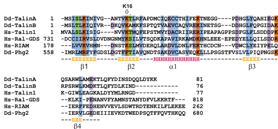
Fig. 1 N-terminal part of Dictyostelium TalinB has a putative RA domain. Alignment of the putative RA domain of Dictyostelium TalinA and TalinB against the RA domains of human Talin1, Ral-GDS, RIAM and Dictyostelium Phg2. The conserved lysine K16 that is mutated in GFP-TalB-K16A is indicated. Structural elements are indicated below for β-sheets (E) and α-helix (H)
